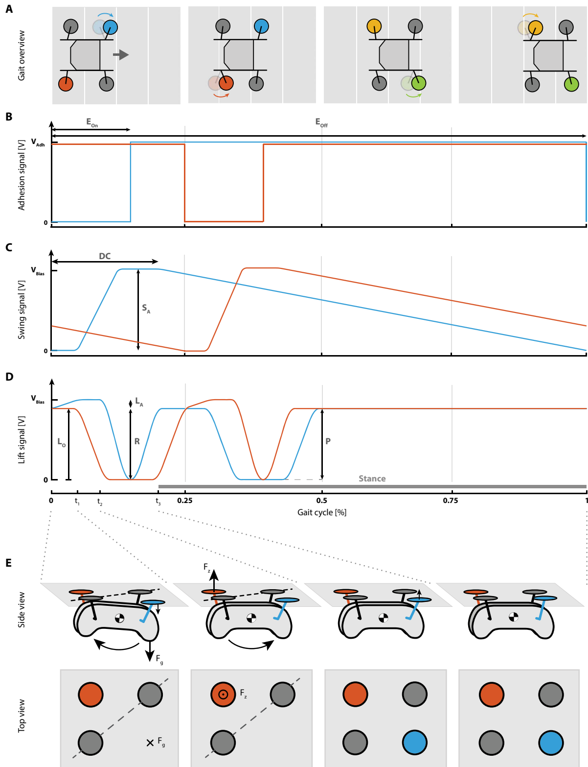
Fig. 3. Modified tripedal crawl gait. (A) Schematic representation of the tripedal crawl gait with individual legs colored. Footfalls are spaced one-quarter cycle apart. (B) Electro-adhesion input voltage for consecutive legs, characterized by the activation ( E_{On} ) and deactivation ( E_{Off} ) timings. Note that the orange signal is artificially offset for clarity. (C) Swing input voltage for the newly designed gait with duty cycle (DC) and swing amplitude S_A labeled. (D) Lift input voltage for the newly designed gait defined by the lift offset ( L_O ), the lift amplitude ( L_A ), reach ( R ), and push ( P ) parameters. (E) Schematics of HAMR-E's pose and gait pattern visualizing the effects of the reach and push parameters during a quarter gait cycle.
